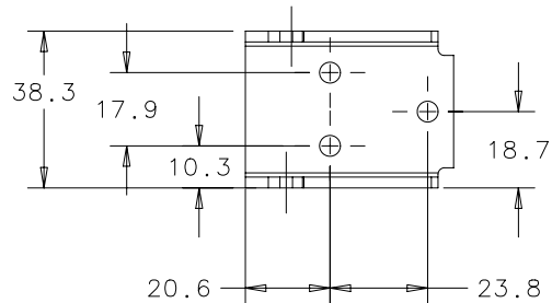
MOUNTING BRACKET
