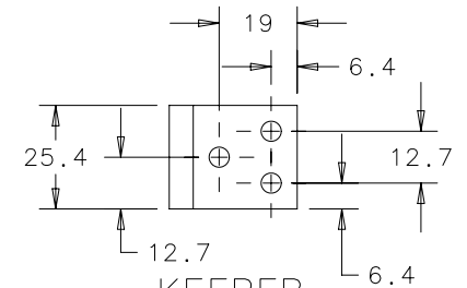
KEEPER
