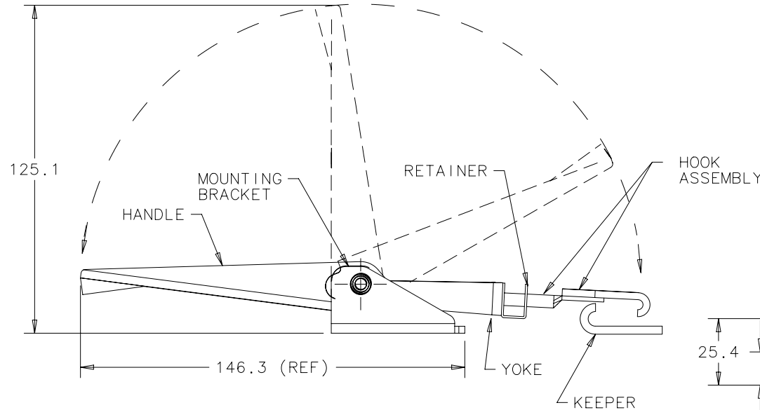
LATCHED POSITION
