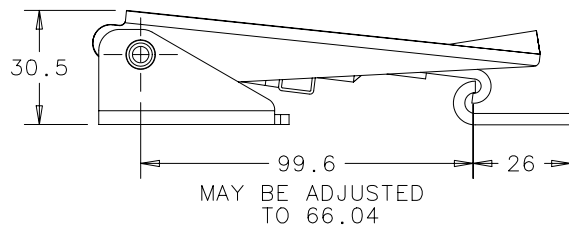
LATCHED POSITION
