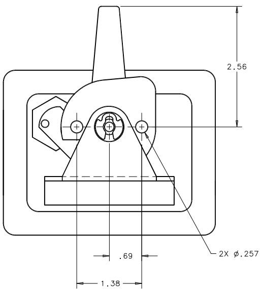
PANEL PREPARATION (WELD)
