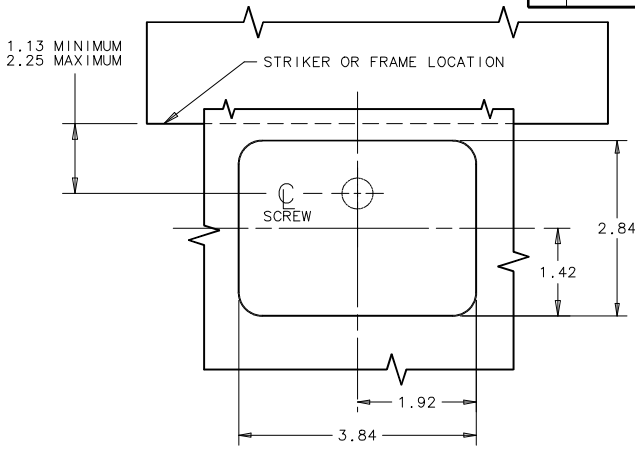
PANEL PREPARATION (WELD)
