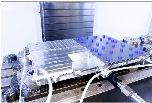
System design Matrix-Plates MPL
