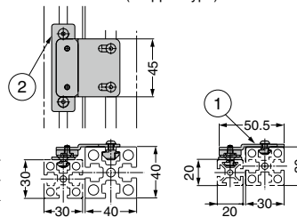
AS-JM-45D (Stepped type)
