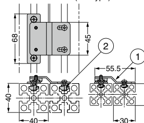
AS-JM-45F (Flat type)
