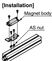
[AS Parts Set] Parts set of brackets, counter plate, screws and AS nuts used for installing to aluminium frame
