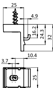
Top Angle Clamp I 40, Slot 8 (Set) Platten-Klemmwinkel I 40, Nut 8 (Set)
