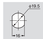
[Cut Out Dimensions]
