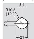
[Cut Out Dimensions]
