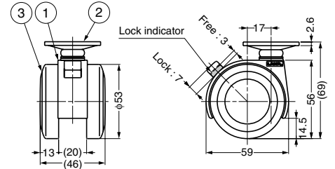
Caster bracket FA55-FIX to lock swivel available (P.740).
