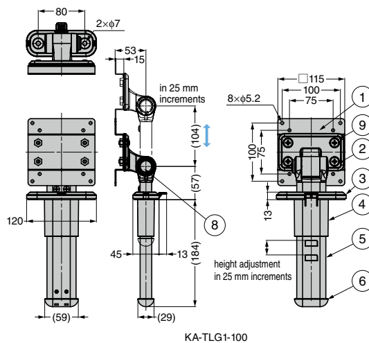
The tilt adjustment of both axes unlocks while the button is pushed.
