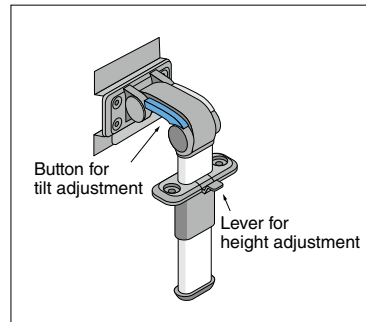
The tilt adjustment of both axes unlocks while the button is pushed.
