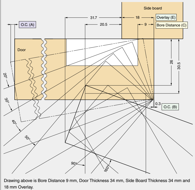
Drawing above is H160-34/18 or H160-C34/18 on to Mounting Plate 100-03A: Bore Distance 9 mm, Door Thickness 34 mm and 18 mm Overlay.
