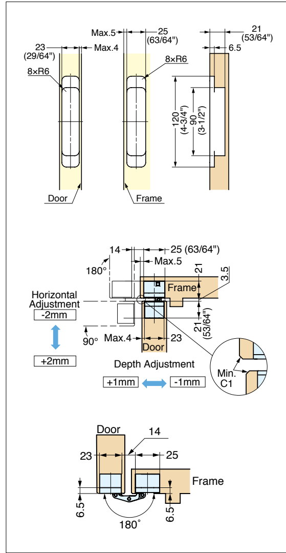
Bore Dimensions
