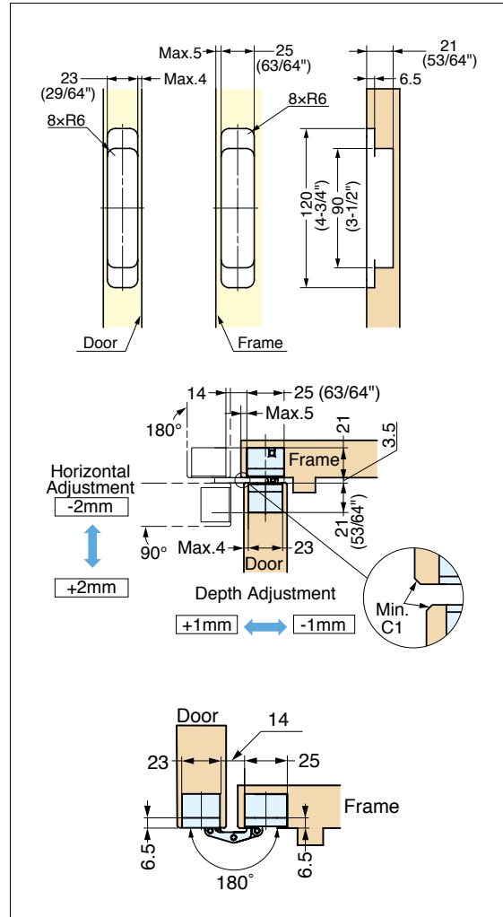
Bore Dimensions
