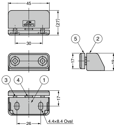
Cover removed
