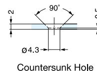
Countersunk Hole
