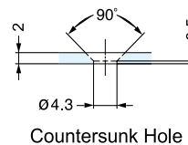
Countersunk Hole
