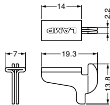
Shelf support
