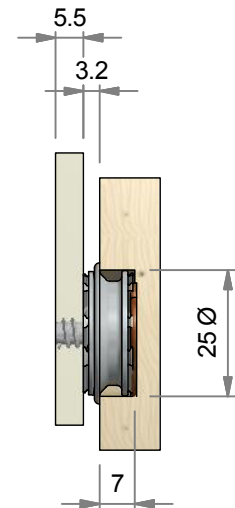
4 Section through recessed installation
