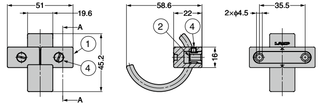
Cross-section View A-A
