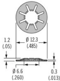
Push-On - Stainless Steel
