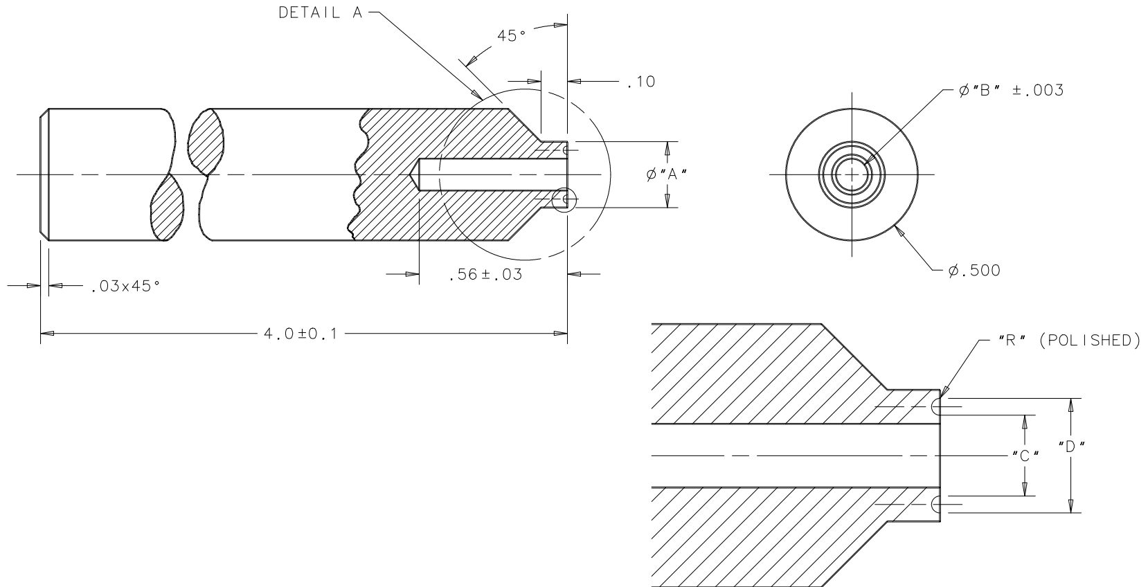
DETAIL A SCALE 4:1
