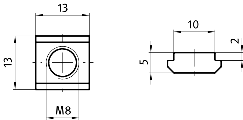
Nutenstein T-slot Nut
