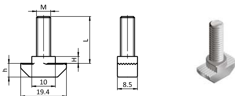
Hammerschraube Hammer Head Screw
