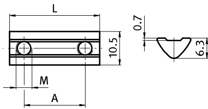
Doppelnutenstein Double T-slot Nut
