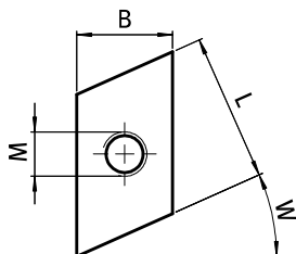
Gewindeplatte Rhombus Threaded Plate Rhombus
