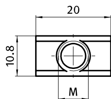
Nutenstein T-slot Nut
